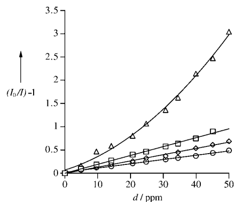
Figure 1. Stern-Volmer plots for the quenching of polysilole luminescence by nitrobenzene ( \circ ), DNT ( \diamond ), TNT ( \square ), and picric acid ( \triangle ).
